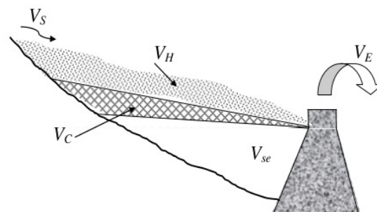
Figure 2. Sketch of sediment control due to sabo structure
