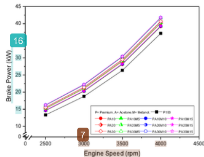
Figure 2. Brake power
