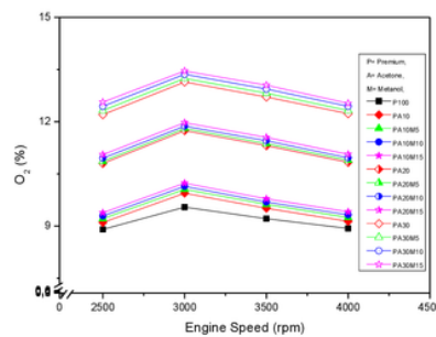
Figure 10. O 2
