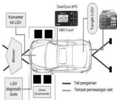
Gambar 2. Experimental setup
