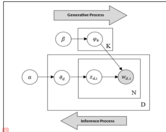
Fig. 1. Graphical model of Latent Dirichlet Allocation
