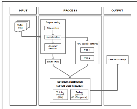
Fig. 2. Sentiment classification process
