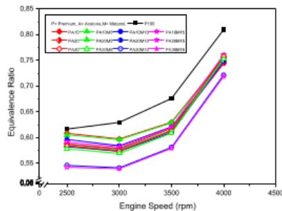
Figure 4. Equivalence ratio
