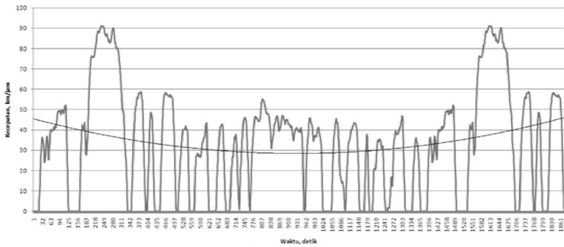
Gambar 3. Driving cycle standar EPA
