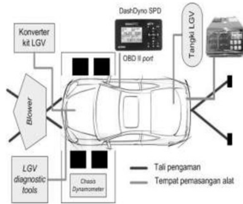
Gambar 2. Experimental setup
