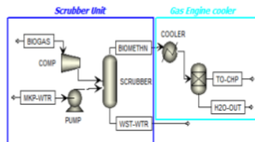
Gambar 3. Biogas Treatment Unit
