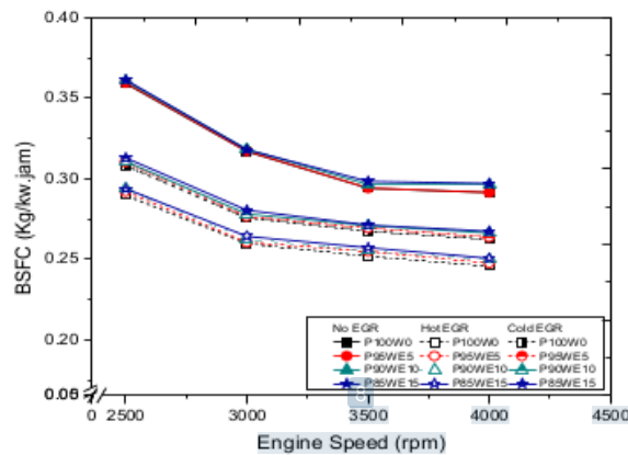
Figure 4. BSFC for various fuel blends with or without EGR at variations in engine speed.
