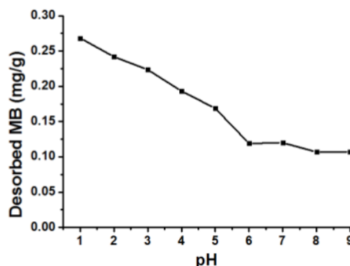
Figure 7. Effect of pH on the methylene blue (MB) desorption process
