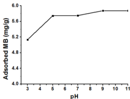
Figure 3. Effect of pH on methylene blue adsorption
