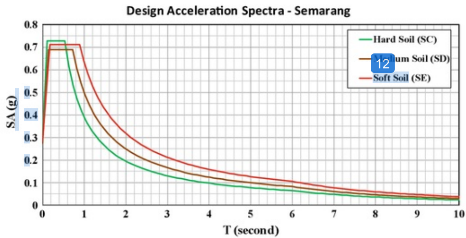
Fig. 4 DARS-2019 of Semarang for site class SC, SD and SE calculated based on S_S and S_I method-3
