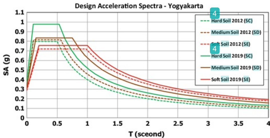
Fig. 8 DARS for Yogyakarta
