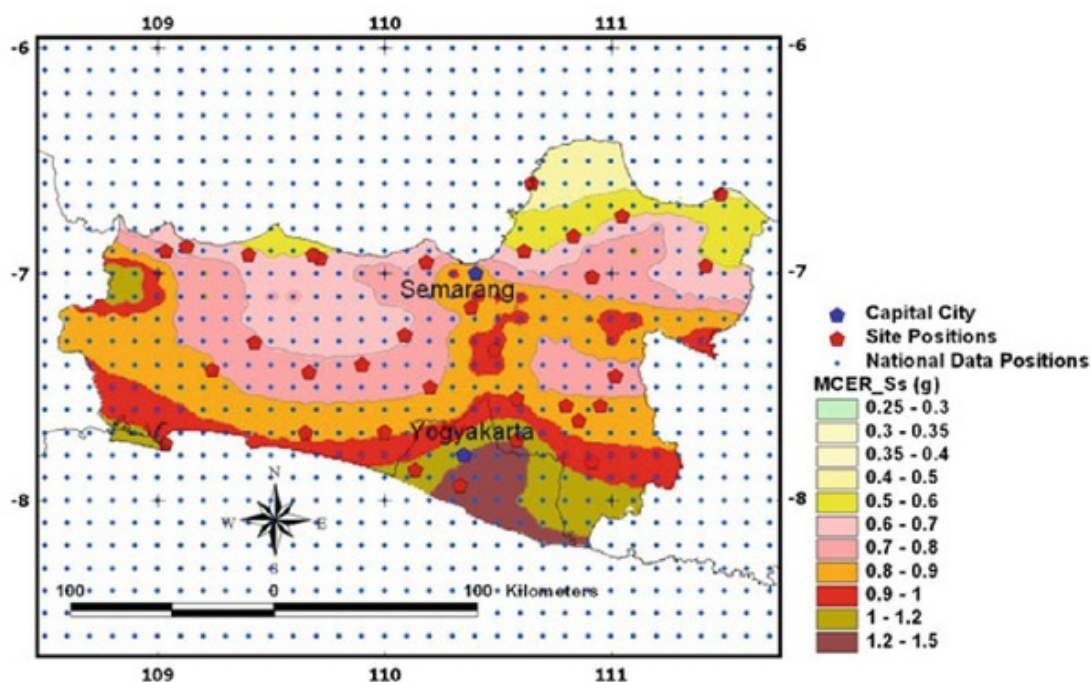
Fig. 1 MCE_R-S_S map of Central Java and Yogyakarta Provinces
