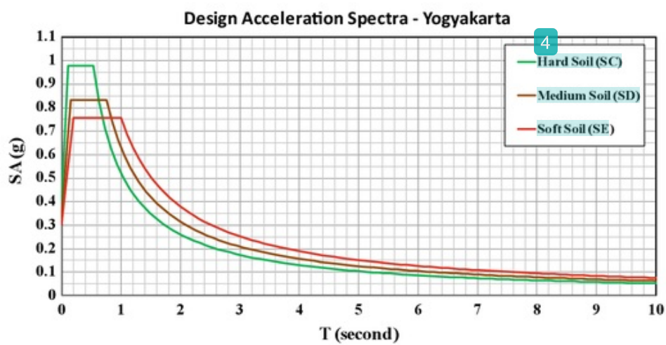
Fig. 3 DARS-2019 of Yogyakarta for site class SC, SD and SE calculated based on S_S and S_I method-3
