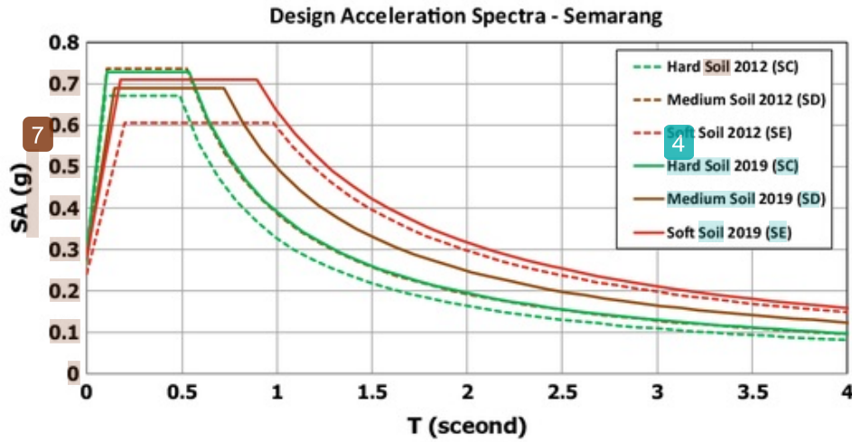
Fig. 7 DARS for Semarang
