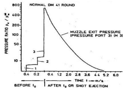
Fig. 2. Reference Pressure graph at initial condition for 7.62 mm NATO G3 rifle.
