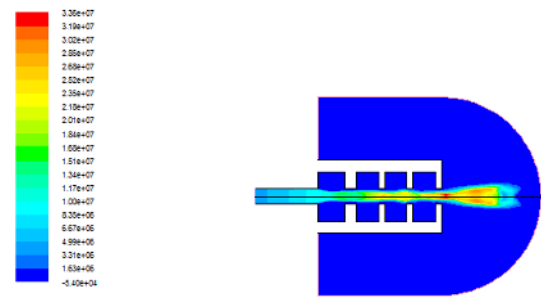
Contours of Total Pressure (pascal) (Time=4.4240e-03)
