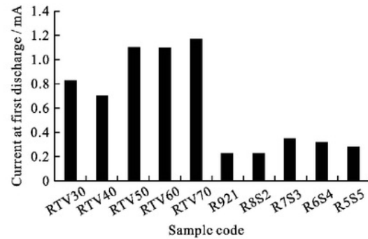
Fig. 11 current at the first discharge
