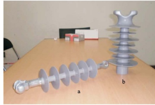
Fig. 1 Polymer insulator (a) suspension and (b) pin-post
