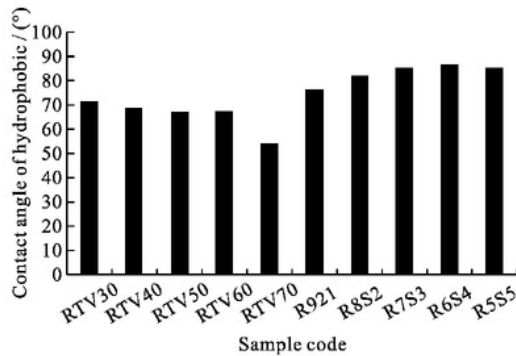
Fig. 9 Characteristics of contact angle of test samples
