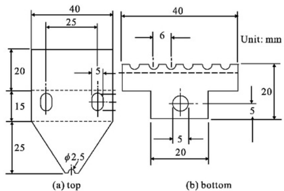
Fig. 4 Top and bottom of the electrodes
