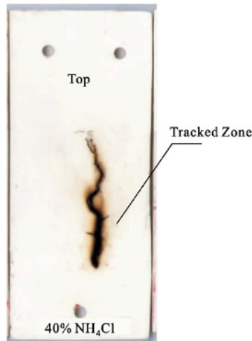
Fig. 12 Tracking formed zone
