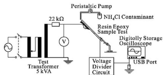
Fig. 6 Schematic diagrams for this test
