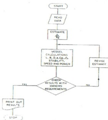
Gambar 1. Flowchart fishing boat design program
