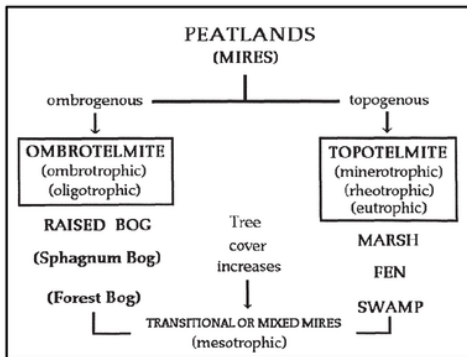
Gambar 2. Diagram lahan gambut (Diessel, 1992)
