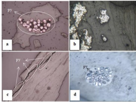
Gambar 4 Fotomikrograf mineral pirit, (a). Framboidal pyrite , (b). Massive pyrite , (c). Epigenetic pyrite , (d). Anhedral pyrite (Win, 2013)
