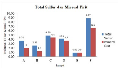
Gambar 8. Hubungan total sulfur mineral pirit.
