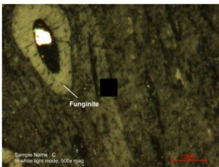
Gambar 6. Fotomikrograf sampel batubara C, sub-maseral teloinertinit (maseral funginite ).
