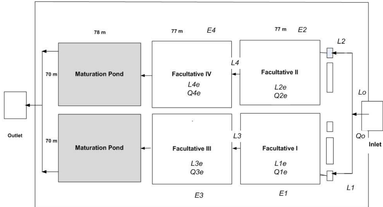
Figure 1: Sewon Bantul Wastewater Treatment Plant
