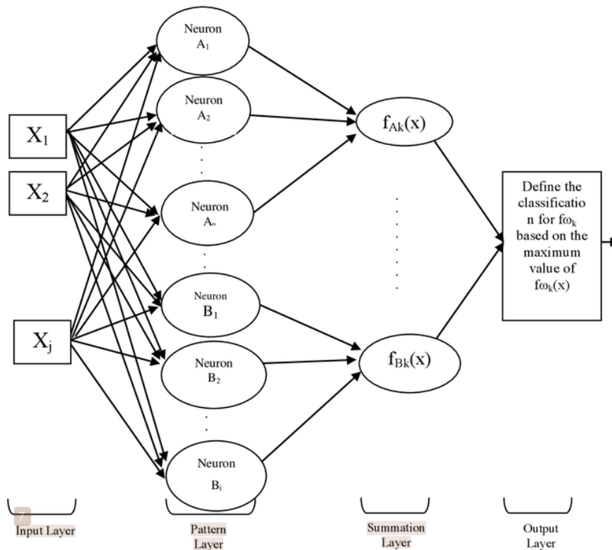
Figure 1. Structure of Probabilistic Neural Network Model
