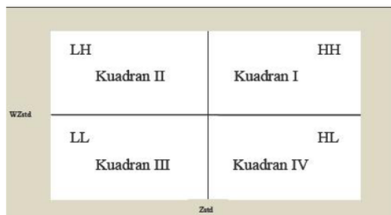
Gambar 2. Moran Scatterplot
