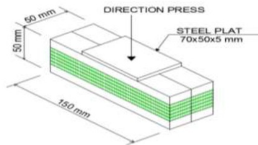
Figure 3 The form of compressive strength test specimen
