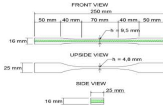
Figure 2 The form of tensile strength test specimen
