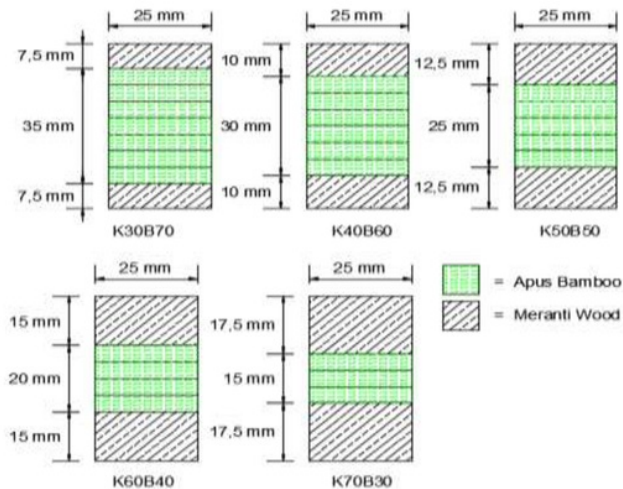
Figure 4 Laminates Composition
