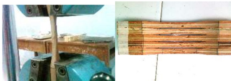
Figure 7 Process of tensile testing and the specimen after the test
