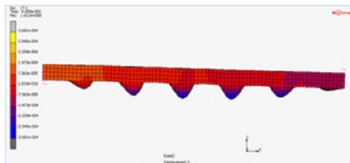
Figure 6 Rectangular pipe buckling
