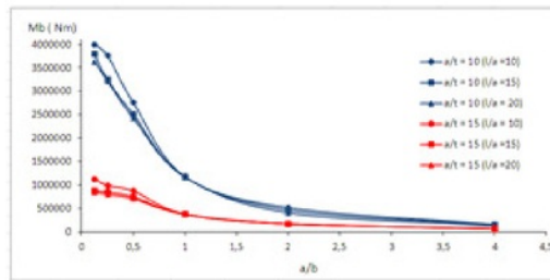
Figure 9 Relationship of buckling moments Iron Holow pipes and a / b
