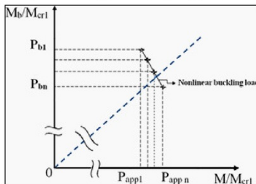
Figure 4 Schematic diagram for estimation of bifurcation moment
