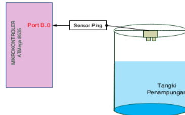
Gambar 2 Alokasi port Sensor PING
