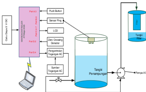
Gambar 1 Blok diagram perancangan Hardware
