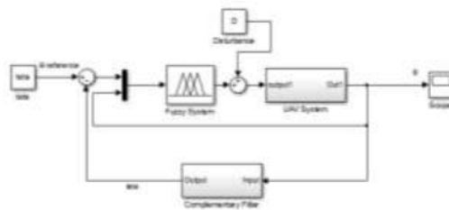
Gambar 5. Diagram blok pengendali sistem fuzzy.
