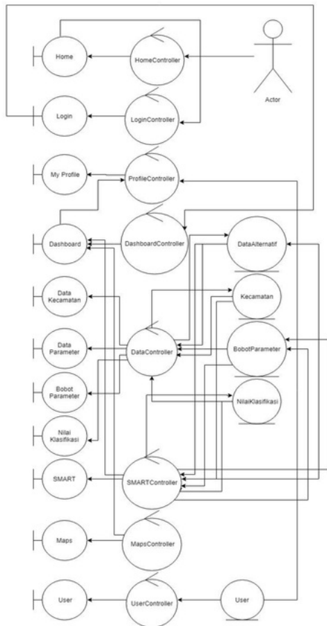
Gambar 3. 2 Entity Control Boundary Diagram
