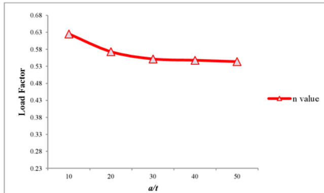
Figure 10: Non-Dimensional Pressure-Thickness Relation Curve of a/b=2
