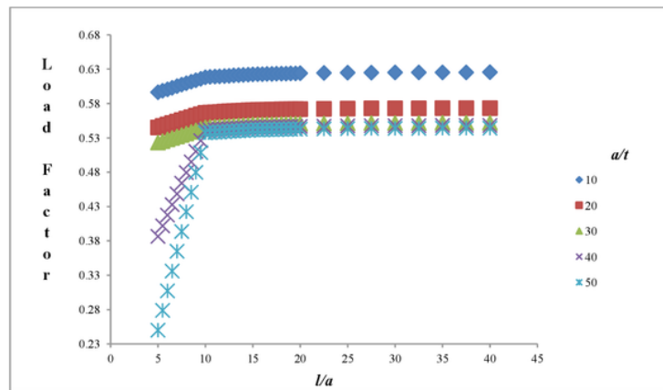
Figure 8: Non-Dimensional Pressure-Length Relation Curve of a/b=2
