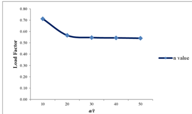
Figure 8: Non-Dimensional Pressure-Thickness Relation Curve of a/b=1
