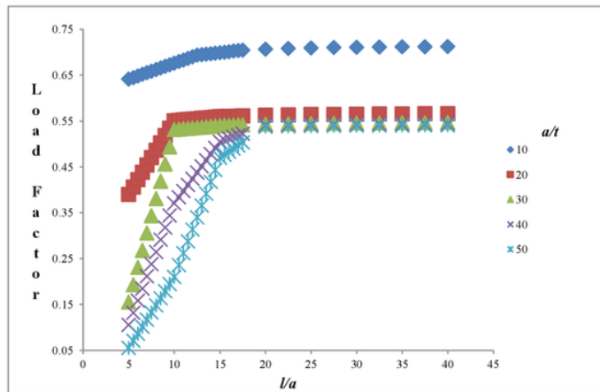
Figure 7: Non-Dimensional Pressure-Length Relation Curve of a/b=1
