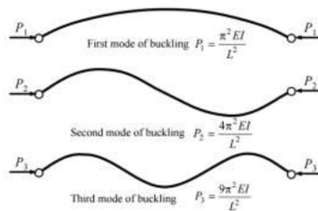
Figure 1: Mode Shape Visualization (Courtesy by Vurg Amit)
