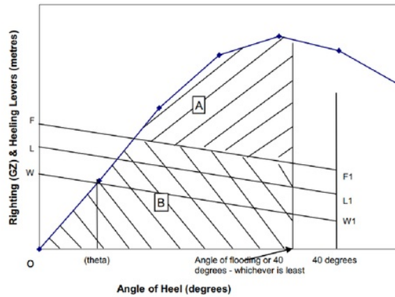
Fig. 5. Illustration of intact stability requirement for Livestock Carrier, [16]
