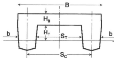
Fig. 3. The basic dimensions of Catamaran, [10]
