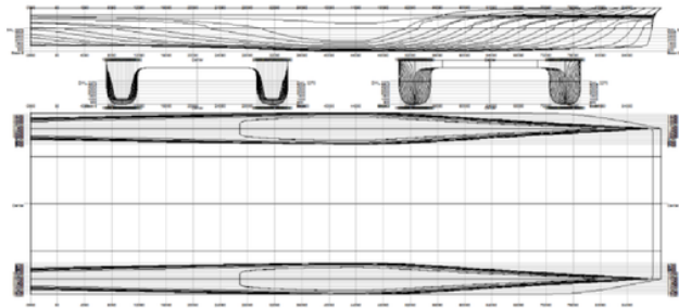
(c) The catamaran concept design
