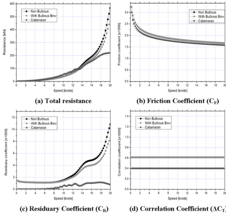
Fig. 4. The total resistance and resistance coefficients of the three hull form
