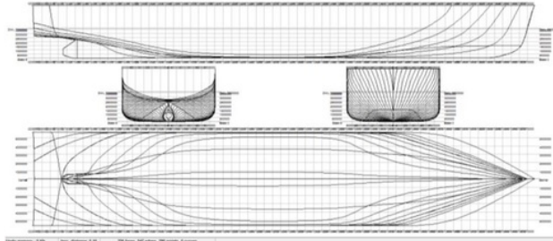
(a) The monohull non-bulbous bow concept design
