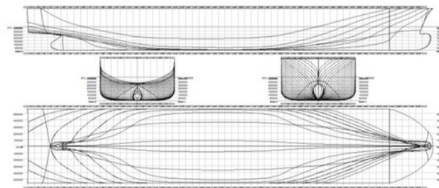
(b) The monohull with bulbous bow concept design
