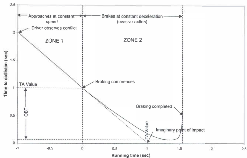
Fig. 4 The relation of TCC and TA Value
