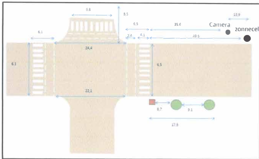
Fig. 6 Intersection configurations and distance references
