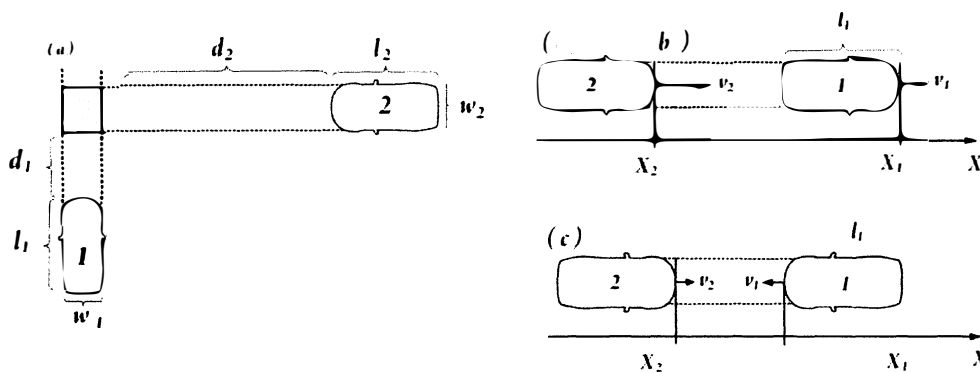
Fig. 3 Calculation of TTC for perpendicular (a) and parallel courses (b, c)
