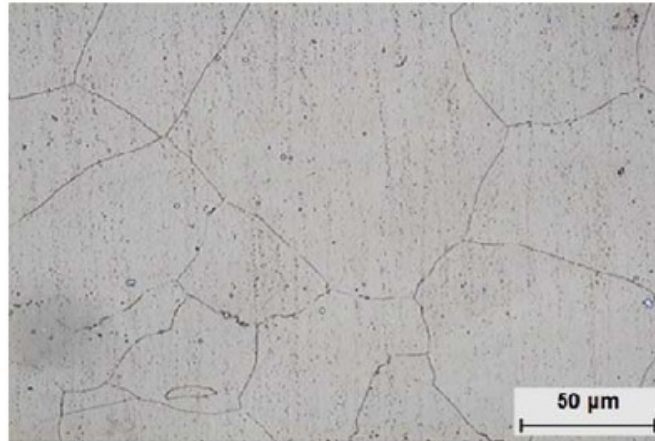
Fig. 1. Metallography of carbides and grain structure in the as-received Alloy 617.
