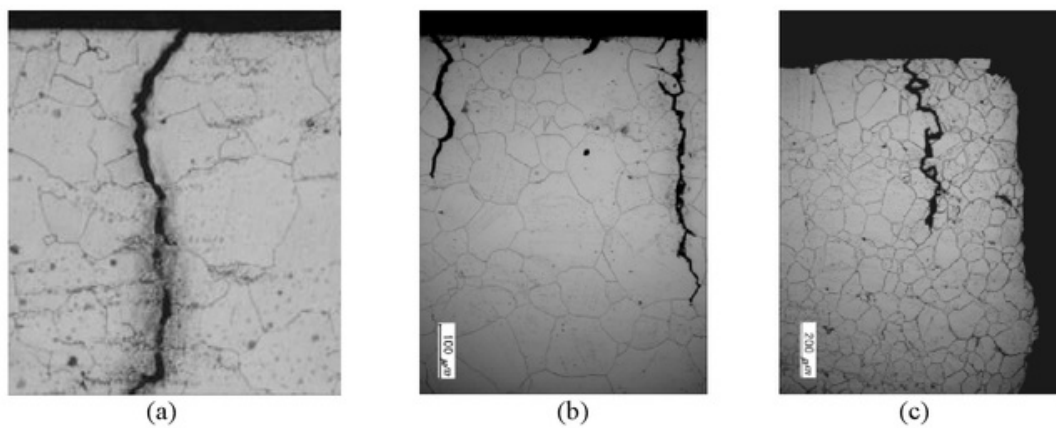
Fig. 3. Micrographs illustrating failure mechanism of Alloy 617 at elevated temperatures: (a) Room temperature; (b) 900°C; and (c) 950°C. The stress axis is from left to right in the plane of the page.
