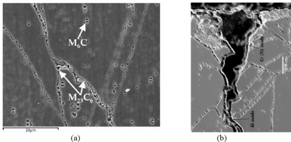
Fig. 4. Typical SEM images of Alloy 617 at high temperature environment illustrating: (a) Precipitates formed in the grain interior and its boundary; and (b) Surface brittle Cr-oxides cracks.
