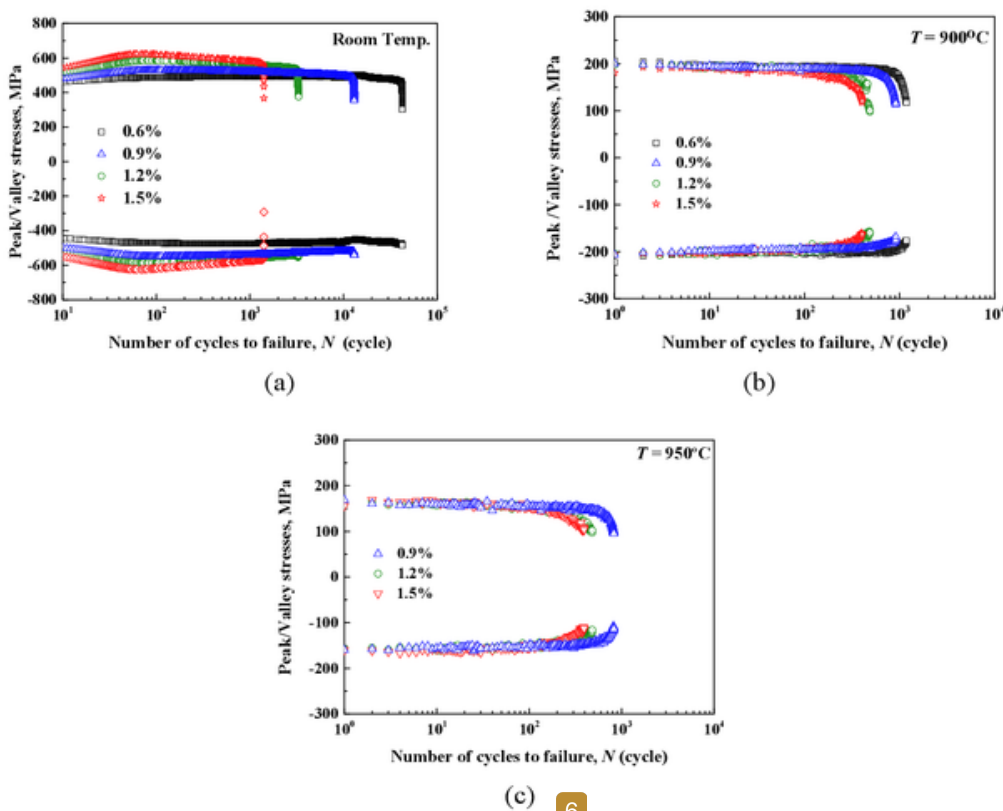
Fig. 2. Peak and tensile compressive stresses response as a function of the number of cycles of Alloy 617 at elevated temperatures: (a) Room temperature; (b) 900°C; and (c) 950°C.
