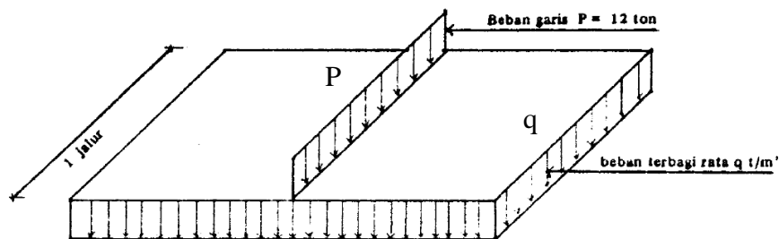
Gambar 2.4 Beban “D”
