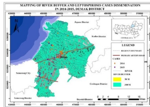
Fig.7. River Buffer and Leptospirosis Cases Dissemination
