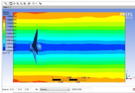
Figure 19. Pressure on the back side at 750RPM
