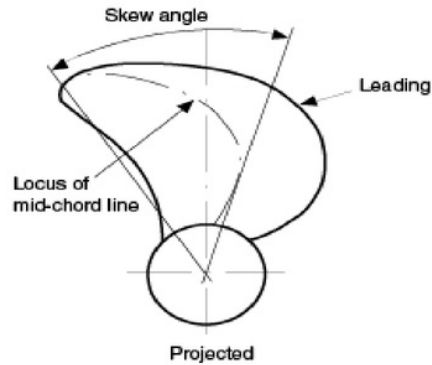
Figure 3. Balanced skew
