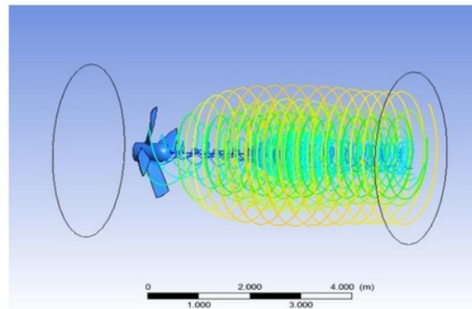
Figure 12. Result model
