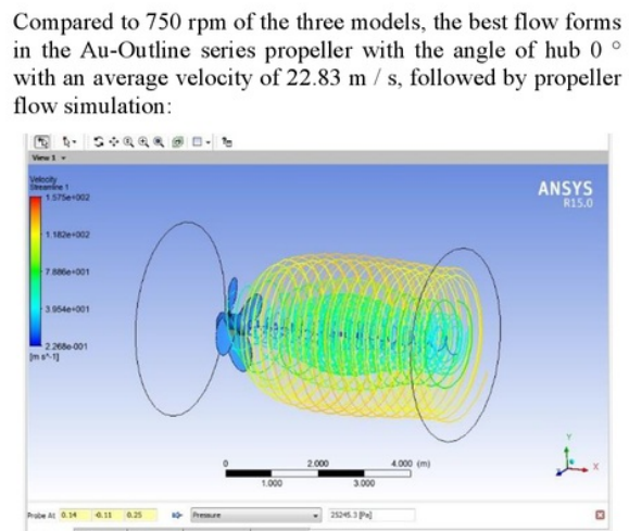
Figure 21. Fluid flows on Au-Outline at 750 RPM
