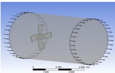
Figure 10. Boundary Set-up
