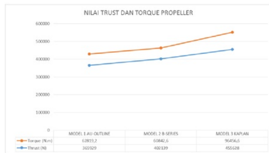
Figure 13. Thrust and Torque Comparison
