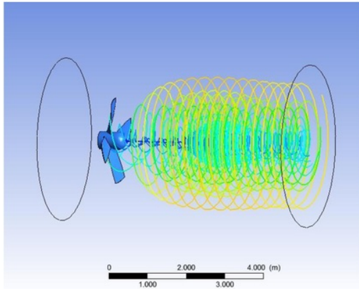
Figure 23. Fluid flows on Kaplan at 750 RPM
