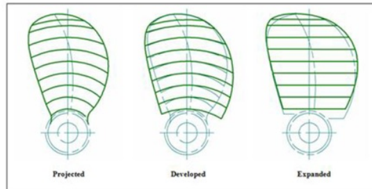
Figure 5. Type Blade Area Ratio.
