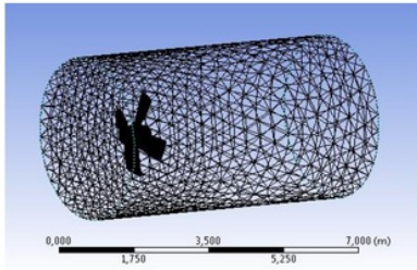
Figure 9. Mesh Stage
