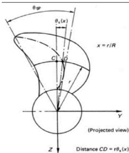
Figure 2. Skew Angle propeller
