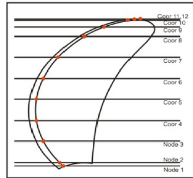
Figure 14. Pressure Coordinates
