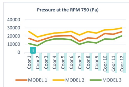
Figure 15. Pressure on Model.
