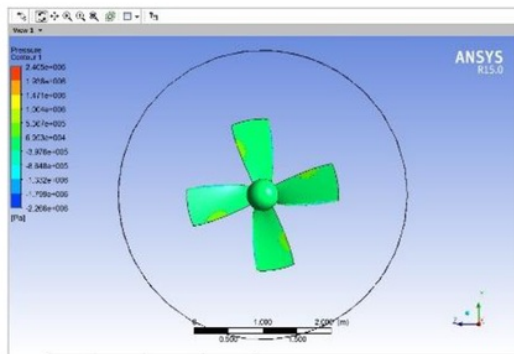
Figure 18. Contour of Kaplan
