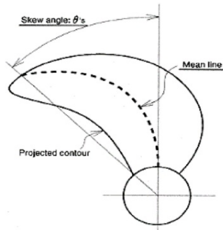
Figure 4. Biased skew
