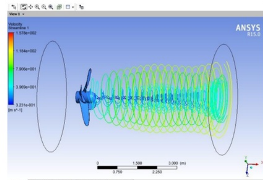
Figure 22. Fluid flows on B-series at 750 RPM
