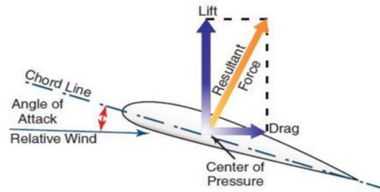
Figure 1. Forces of propeller foil
