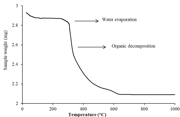
Figure 1. Thermogravimetric analysis of petung bamboo leaf temperature of 30 – 1000°C
