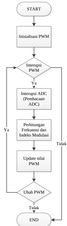
Gambar 5. Flowchart program UPWM
