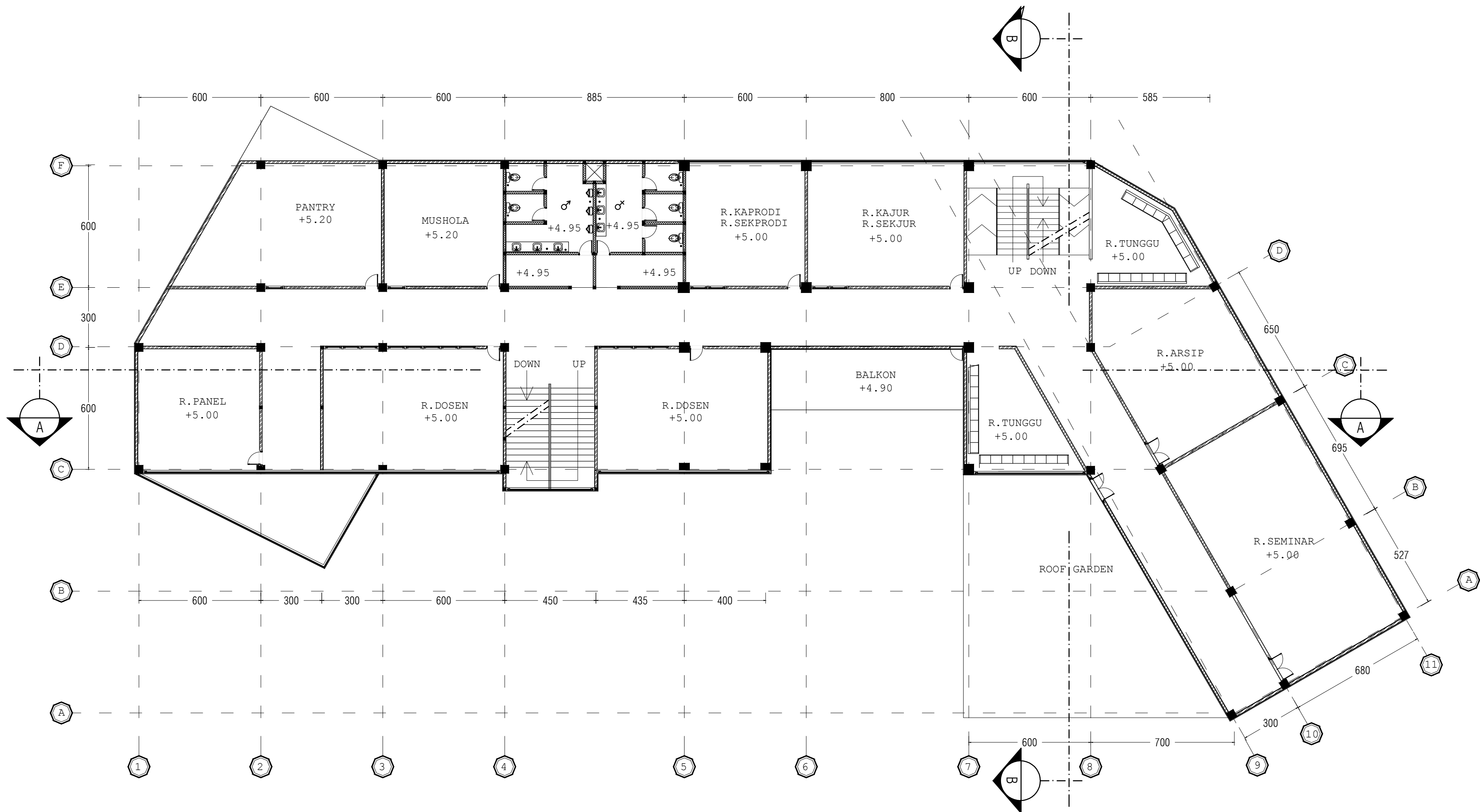
02 DENAH LT.2 REF SKALA 1:150
