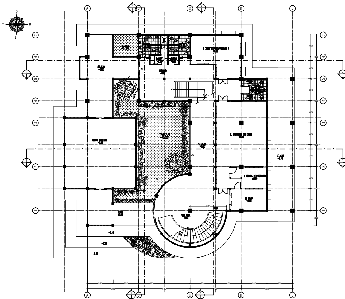
DENAH LANTAI 1
