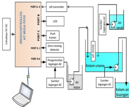
Gambar 6 Rancangan hardware pengendali pH air.
