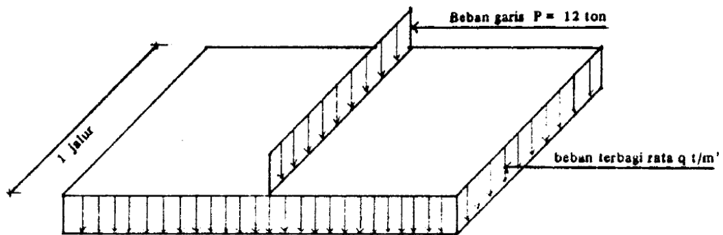
Gambar 2.2 Beban “D”
