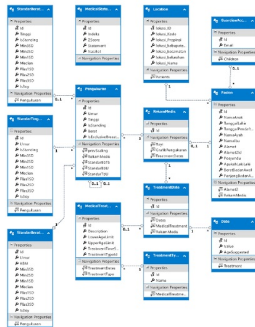
Gambar 6. Entity Data Model
