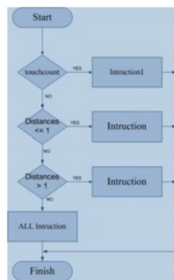
Gambar 17. Flowchart PinchZoom
