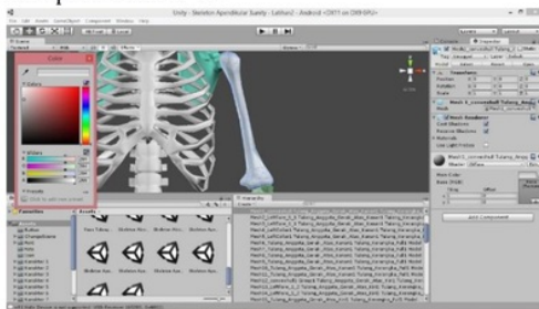
Gambar 13 Setting Colour
