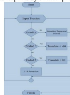
Gambar 19 Flowchart ShiftObject
