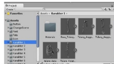
Gambar 10 Export Objek
