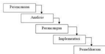
Gambar 1 Waterfall
