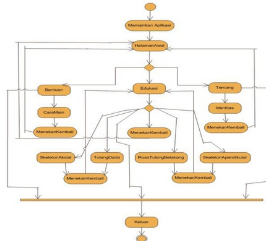
Gambar 7 Diagram Activity
