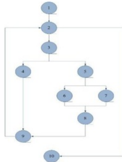
Gambar 16. Flowgraph SwipeObject
