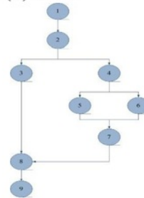
Gambar 18 Flowgraph PinchZoom
