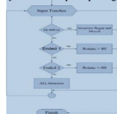
Gambar 15. Flowchart SwipeObject
