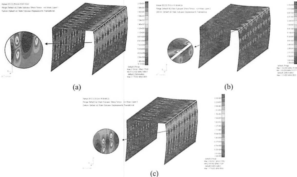
Fig. 3. (a) The stress distributions on the bottom layer; (b) The stress distributions on the second layer (polyurethane core); (c) The stress distributions on the third layer (FRP top layer)
