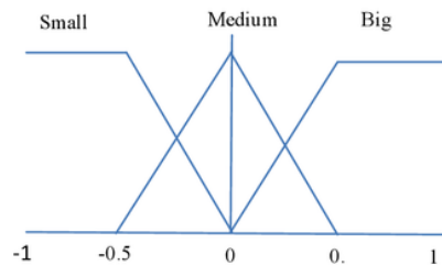
Figure 3. Membership function with input is delta error
