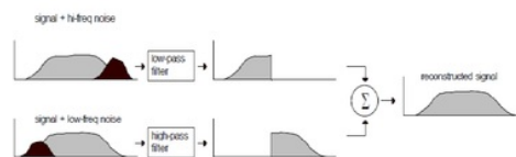
Figure8. Principle of Complementary filter.
