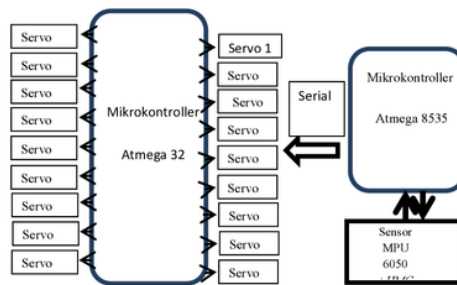
Figure 10. Diagram blok of hardware system
