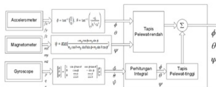
Figure9. Diagram of complementary filter
