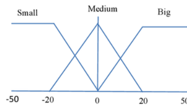
Figure 2.membership function with input is error.
