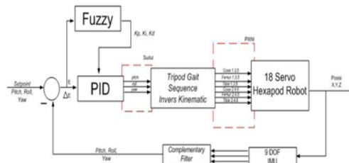
Figure 1. Blok diagramcontroller
