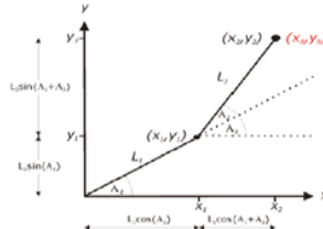
Figure 4. Graphic representation of legged robot
