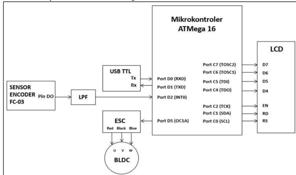
Fig. 2: microcontroller port allocation
