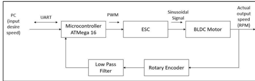
Fig. 1: block diagram hardware design
