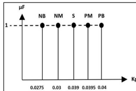
Fig. 6: membership function for Kp
