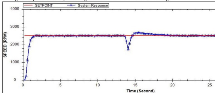
Fig. 15: system response for momentary disturbance
