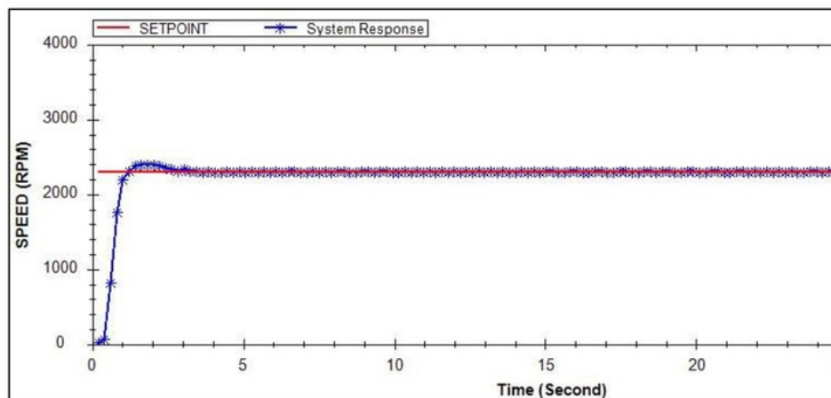
Fig. 10: system response for 2300 RPM use PID controller
