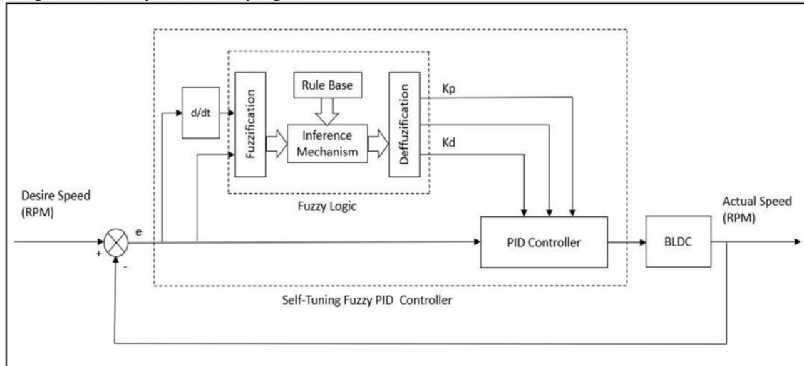
Fig. 3: block diagram control design
