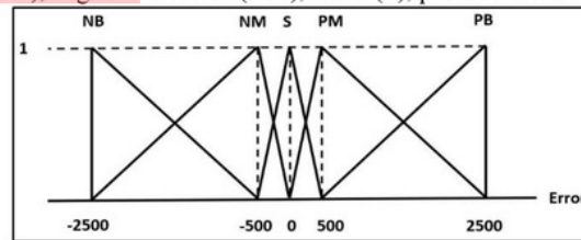
Fig. 4: membership function for error
