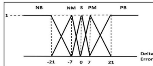
Fig. 5: membership function for delta error
