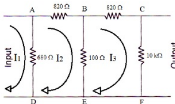
Fig. 3. Voltage divider circuit
