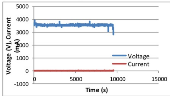
Fig. 5. Relationship between voltage and current in sample 1
