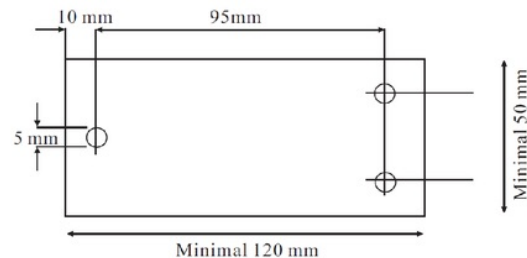
Fig. 1. Size and dimension of test sampel.[8]
