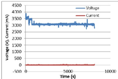
Fig. 6. Relationship between voltage and current in sample 2
