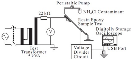
Fig. 2. Leakage current measuring system [8]
