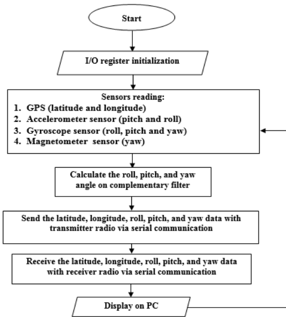
Fig. 3. Main program flow diagram
