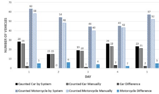
Fig. 7. Comparison of counted vehicles by system with counted vehicles manually from 08.00-14.00 for five days
