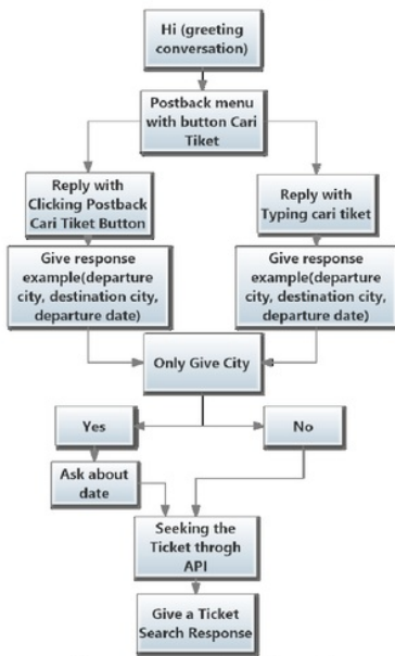
Figure 3 Conversational Flow [6]
