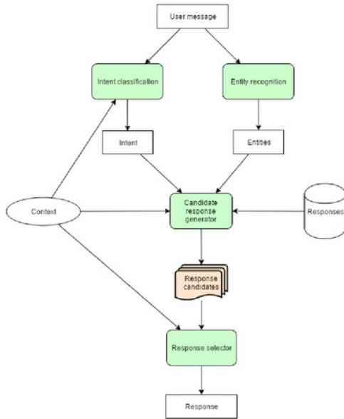
Figure 2 Chatbot Architecture [6]
