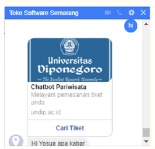
Figure 7 CUI Interaction
