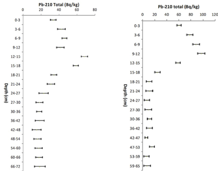
Fig. 3. Total ^{210}\text{Pb} versus depth of the TW2 core (left) and TW3 core (right), decay trend.
