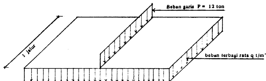
Gambar 2.2 Beban "D"
