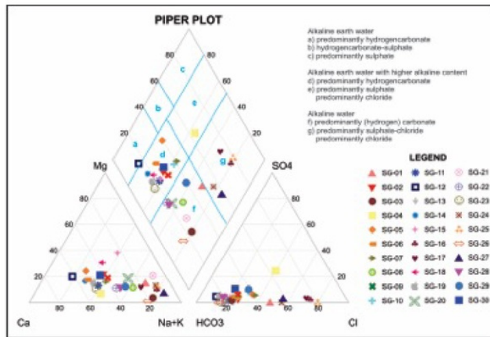
Fig. 5 Piper plot showing the groundwater facies.
