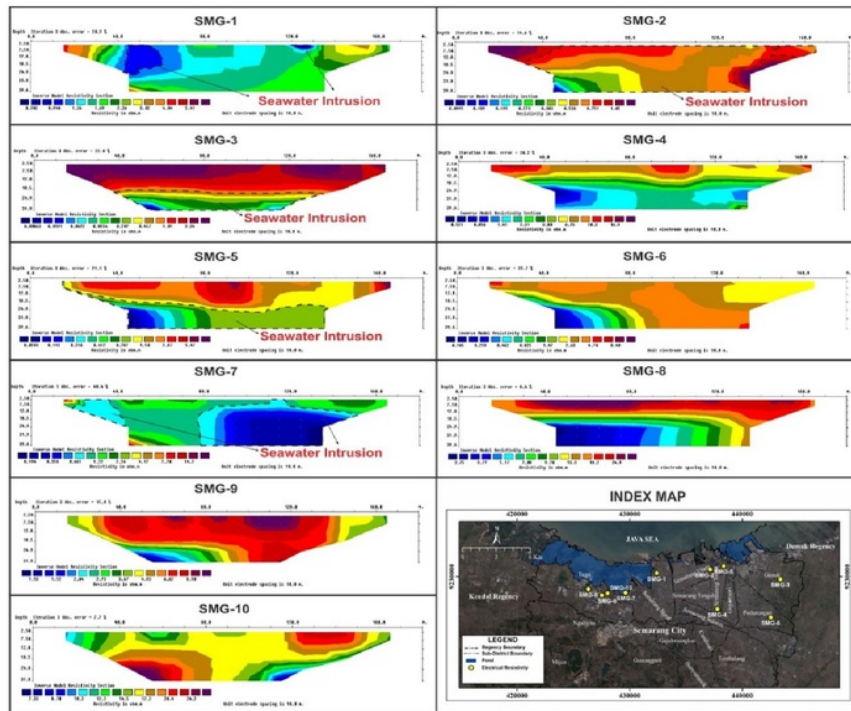
Fig. 3 Inverse model resistivity section of Geophysical survey.
