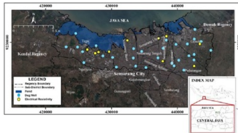
Fig. 2 Geophysical survey (yellow dots) and hydrogeological mapping points (blue dots).
