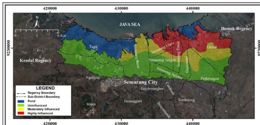
Fig. 6 Seawater intrusion zones
