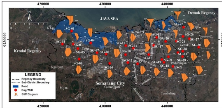
Fig. 4 Stiff diagram showing the distribution of major cations and anions content.
