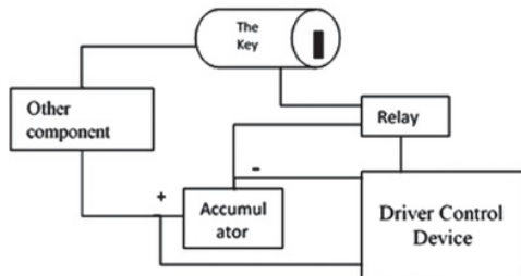
Fig. 3. Deployment of driver control into motorcycle main power.
