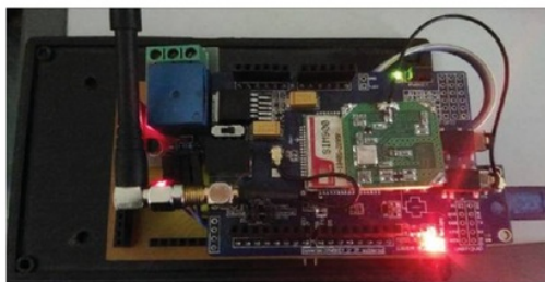
Fig. 2. Driver control equipment.
