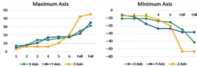
Fig. 4. Maximum and minimum axis of motorcycle's fall.
