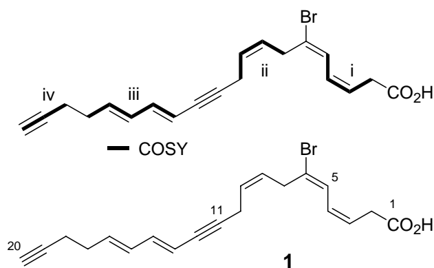
Figure 1. Structure of Compound 1 .
